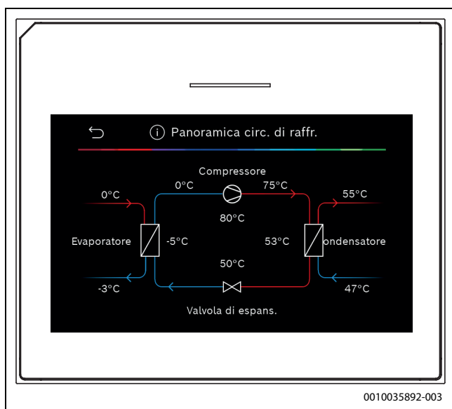
Fig. 10 Panoramic view of the refrigeration circuit
